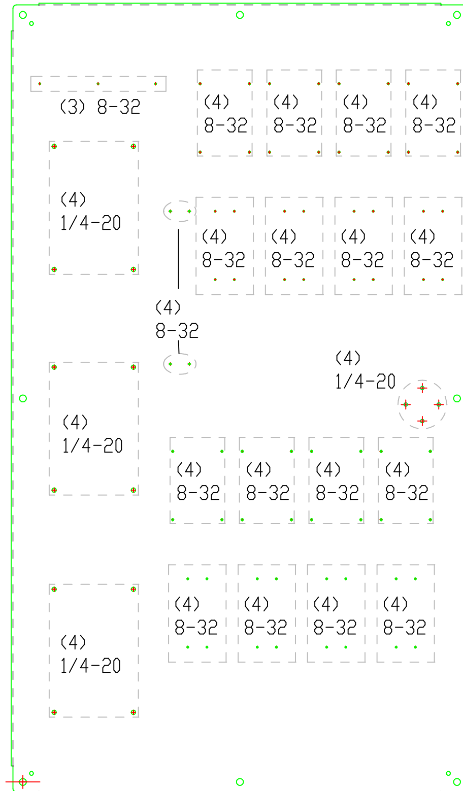
SUBPANEL FRONT VIEW typ.
