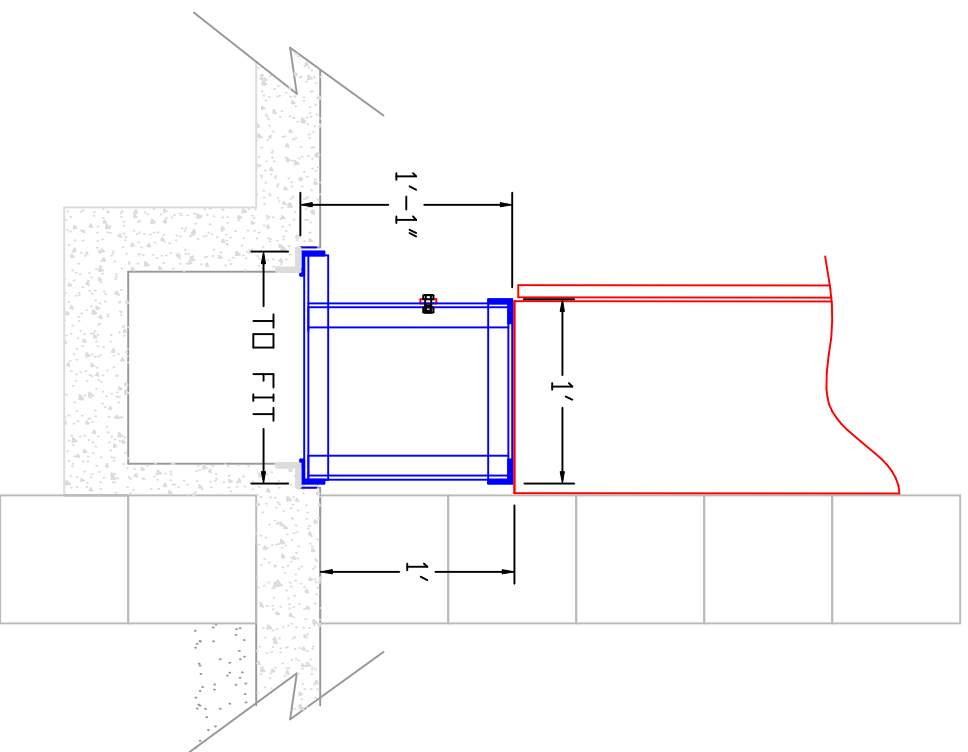
SIDE VIEW
