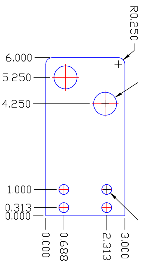
PART A: PIPE BRACKET 3/16" X 3" STEEL PLATE
