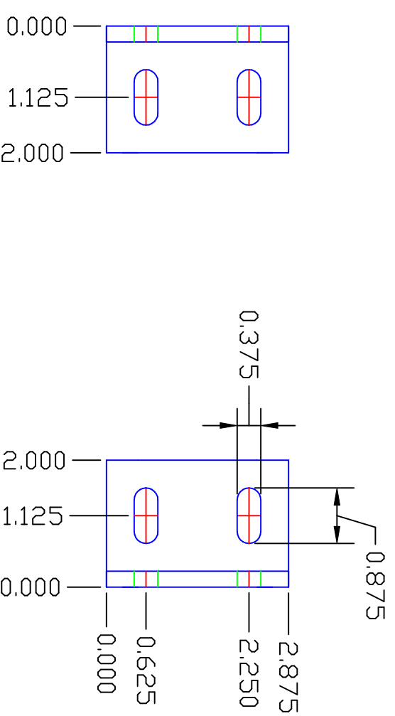
PART B: ADJUST ANGLE 2" X 2" X 3/16" STEEL ANGLE
